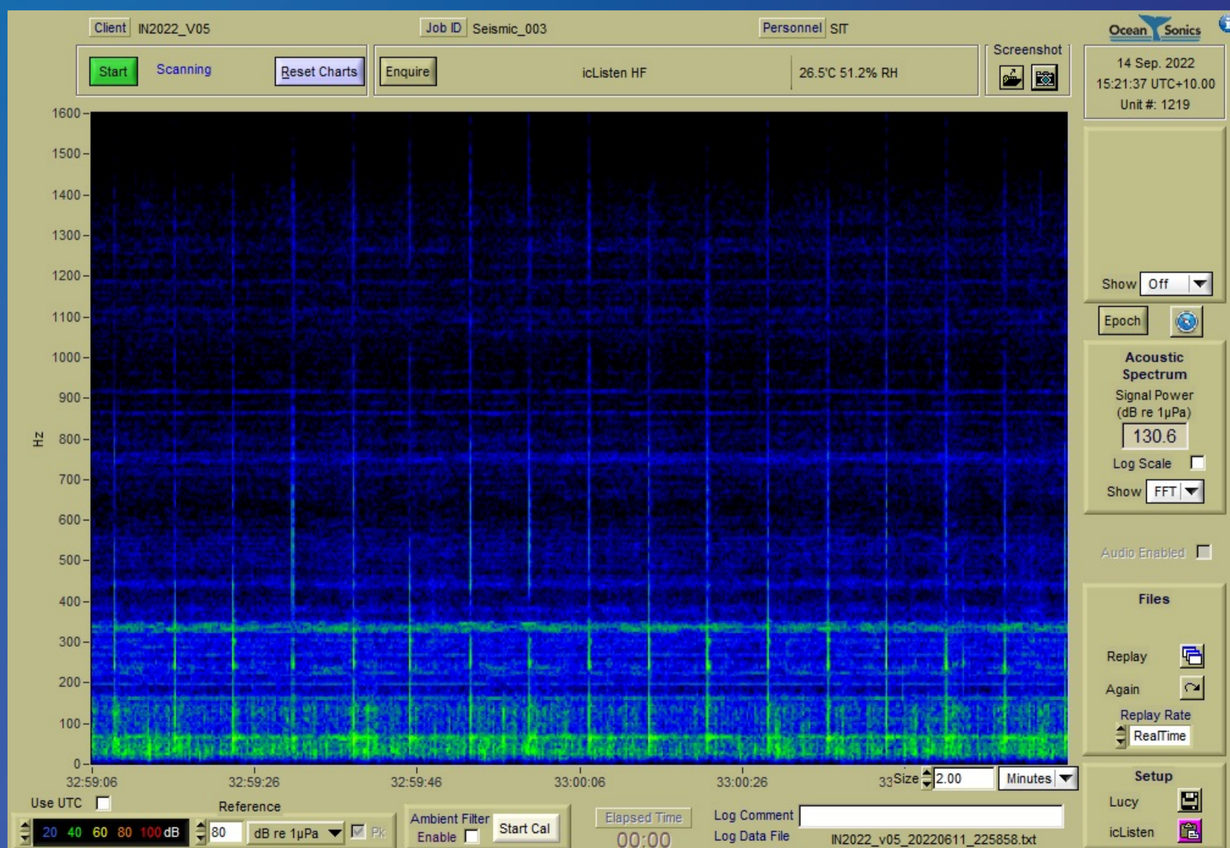
Lucy Software - spectrum of two seismic air guns towed behind the vessel
